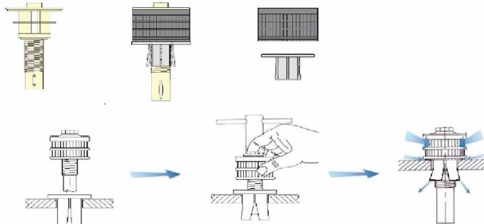
1 1/2" nozzle
